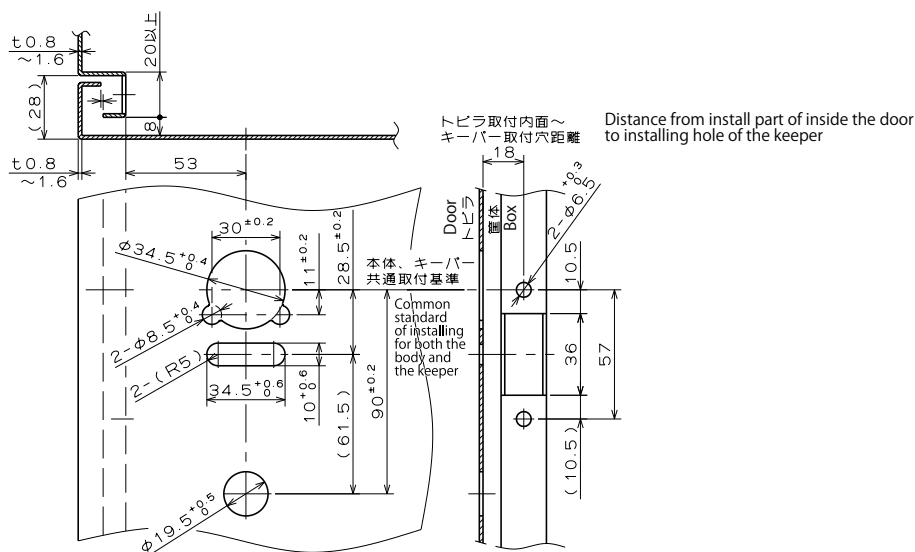
Figure showing dimensions of mounting door and box 取付扉、筐体形状説明図 LL-0031の場合、左右逆 Please consider as reverse left and right in case of using LL-0031
