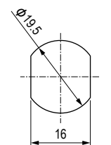
取付穴図 Hole for Installation
