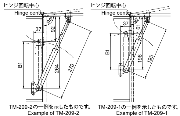
図2取付例 Fig.2. Installation Layout
