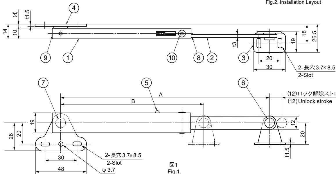
図2取付例 Fig.2. Installation Layout
